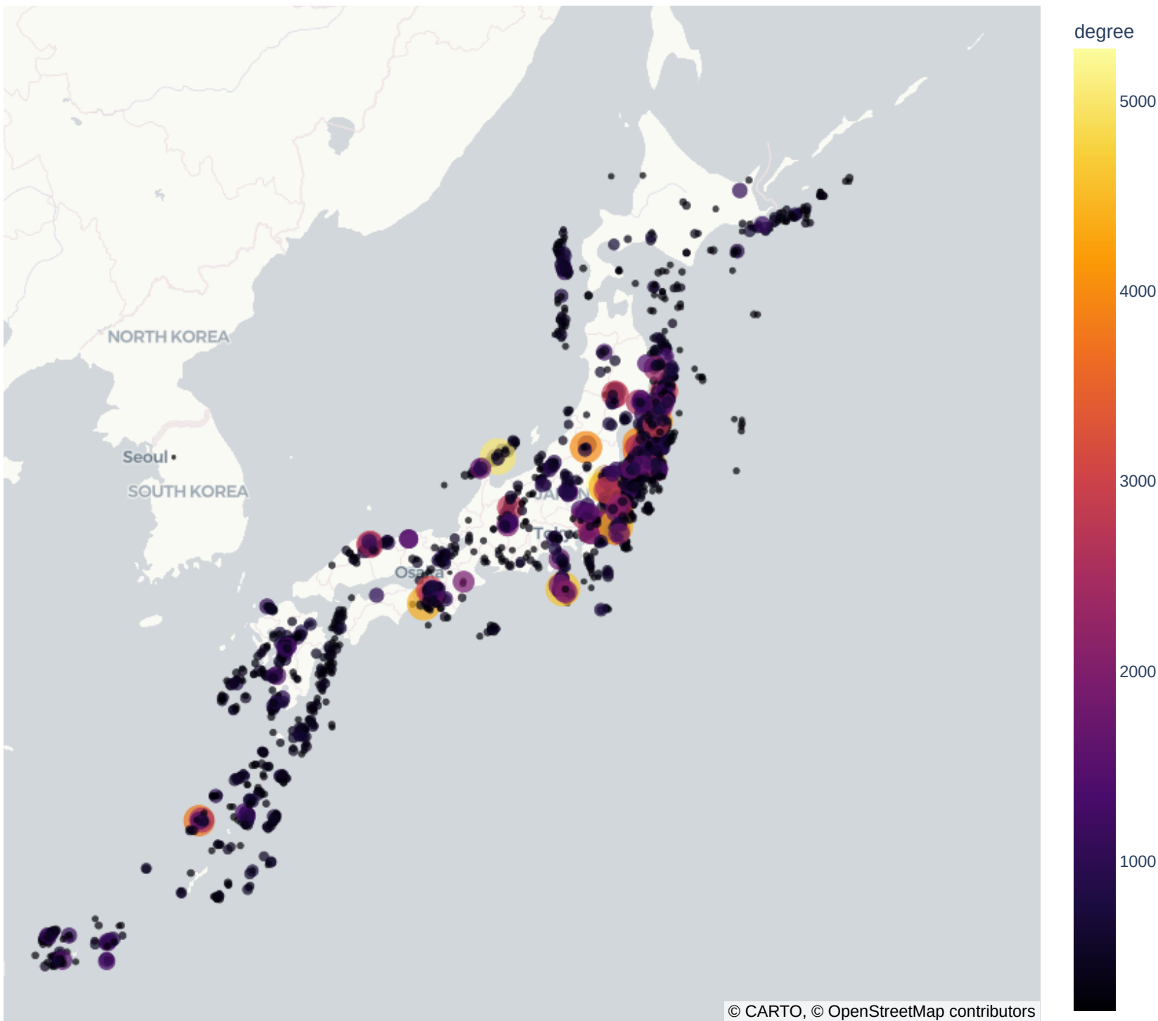
Abe-Suzuki Network Hubs: Top 2% Most Active Seismic Cells — Japan (10x10x10 km)
