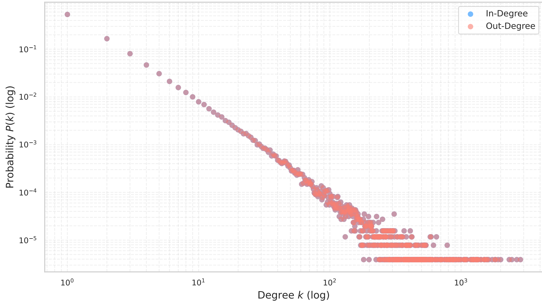
In vs Out Degree Distribution: Abe-Suzuki Japan (5 km)
