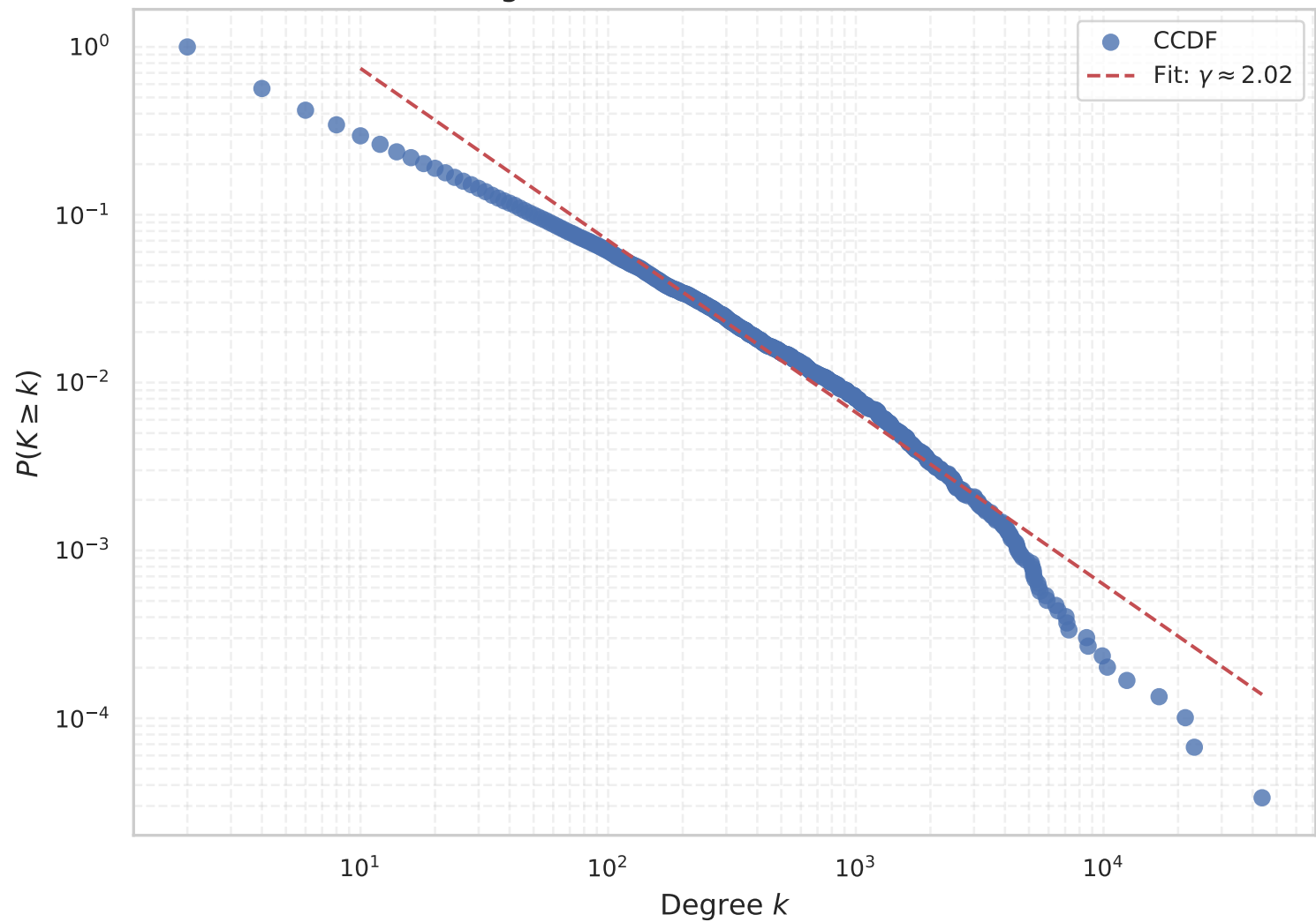
CCDF Degree Distribution: Abe-Suzuki 10 km
