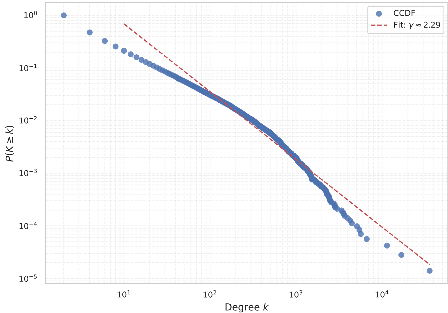
CCDF Degree Distribution: Abe-Suzuki 5 km
