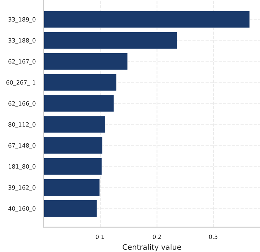
Degree (active cells)
