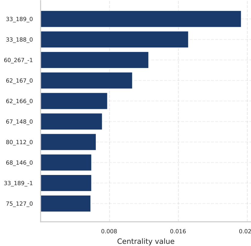
HITS Authority (seismic destinations)
