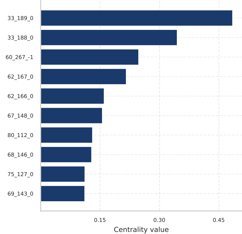
Eigenvector (rich-club core)
