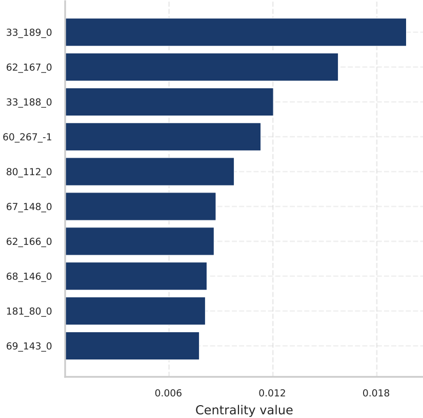
Katz (all-path influence)
