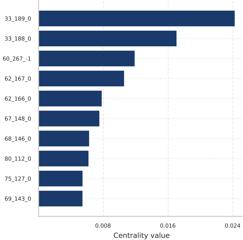
HITS Hub (seismic triggers)
