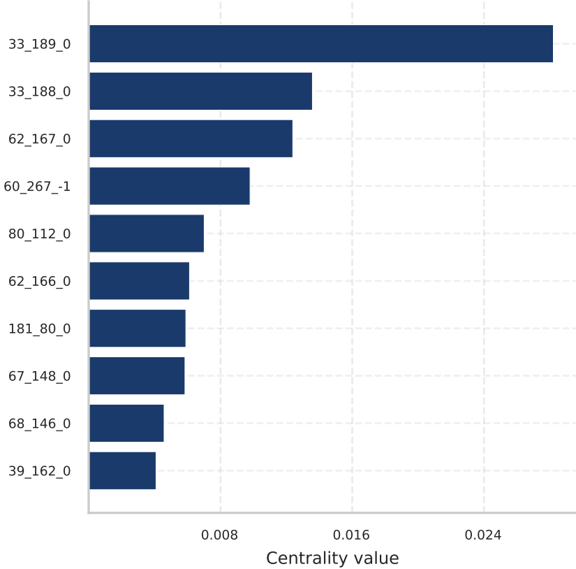
PageRank (stress sinks)
