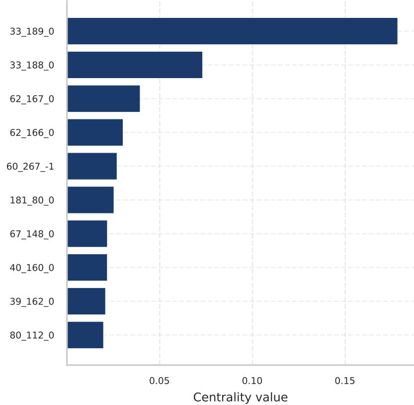
Betweenness (fault bridges)
