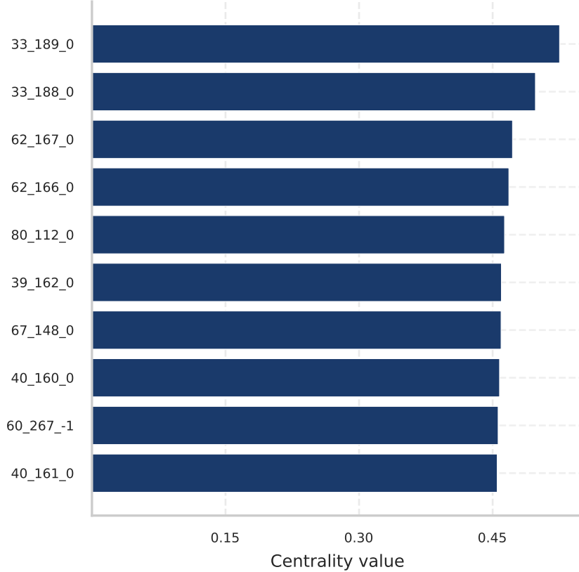
Closeness (global spread)
