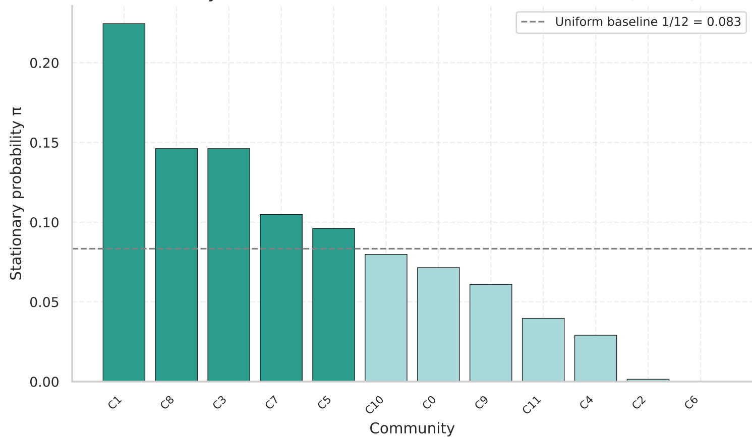
Stationary Distribution of Seismic Flow — Abe-Suzuki US (10 km)
