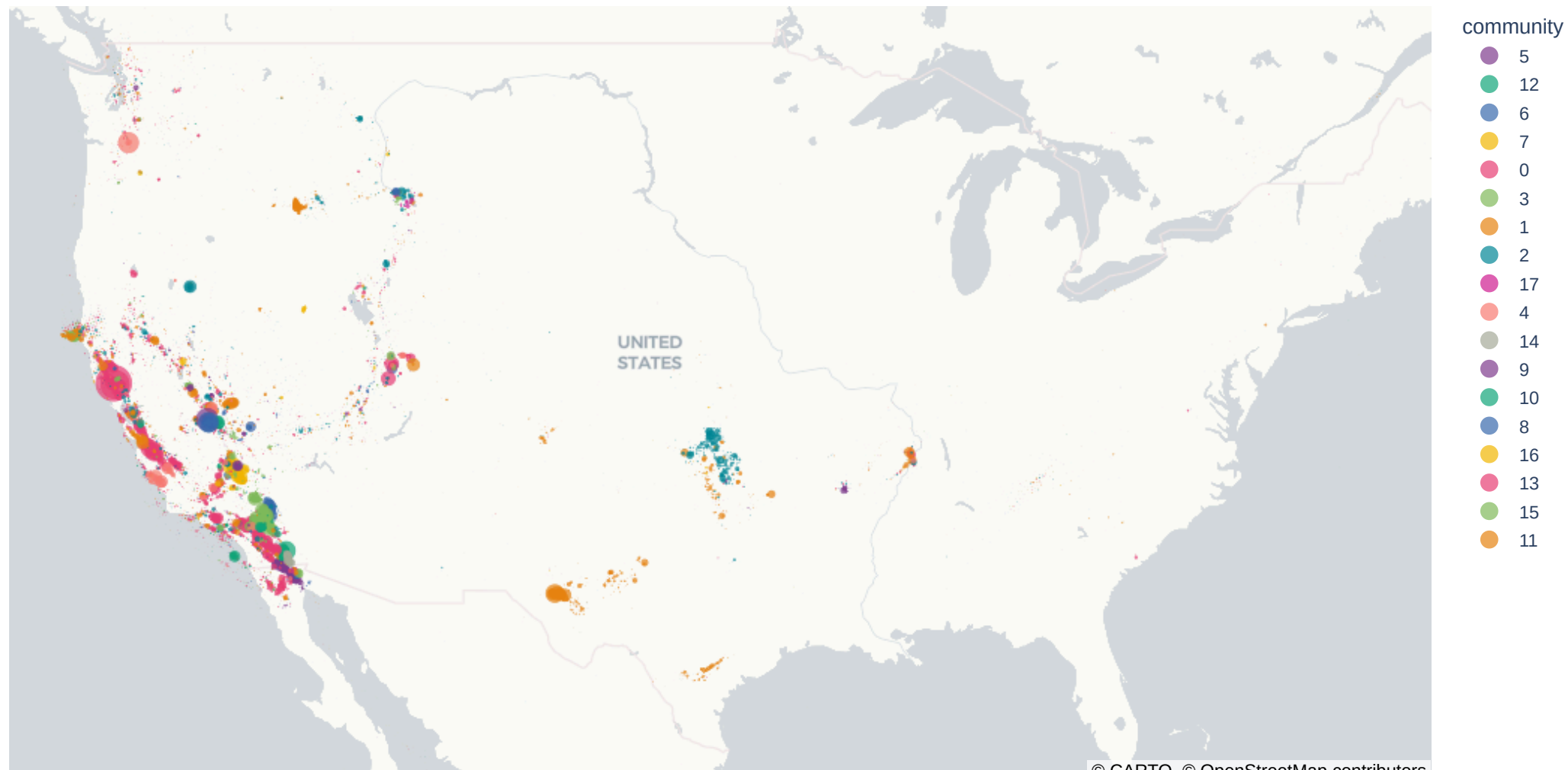
Seismic Communities — Directed Louvain (Leiden) (18 communities \geq 50 nodes) — Abe-Suzuki US (10 km)
