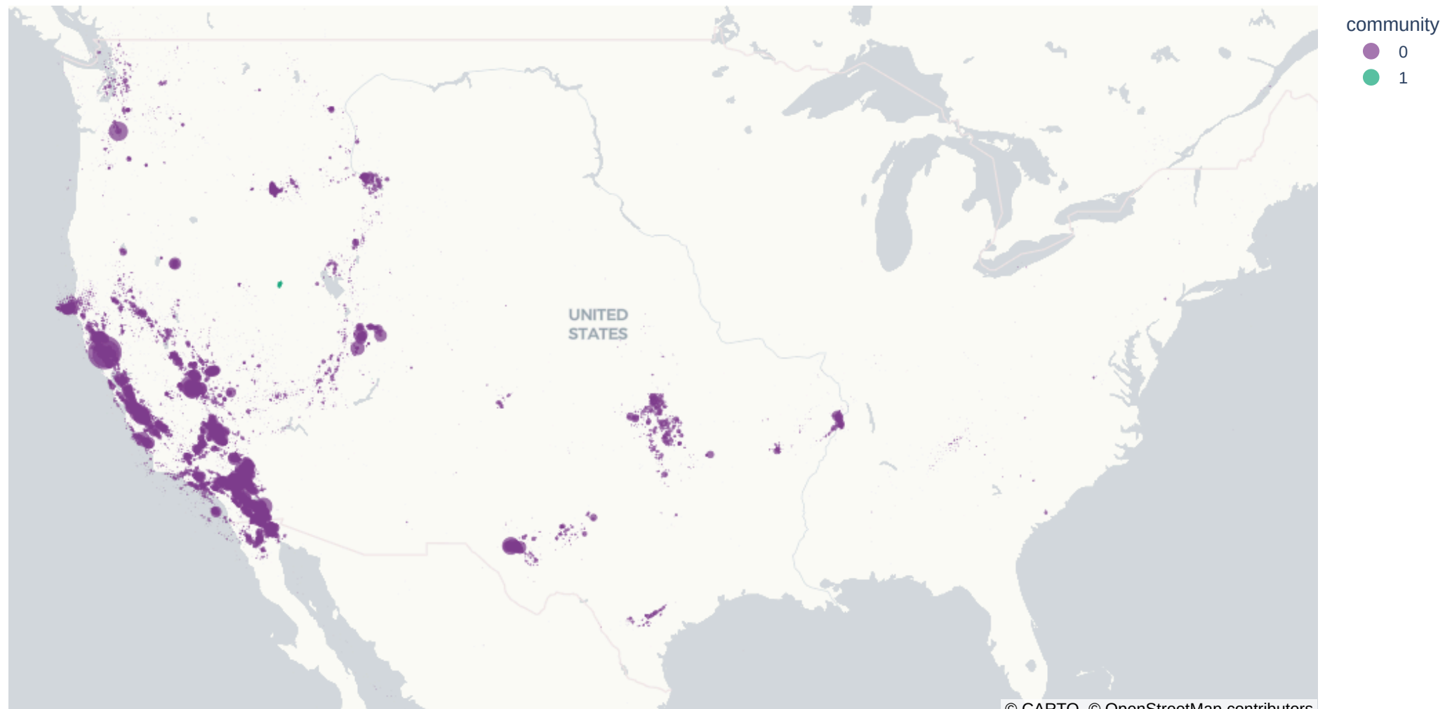
Seismic Communities — InfoMap (2 communities \geq 50 nodes) — Abe-Suzuki US (10 km)
