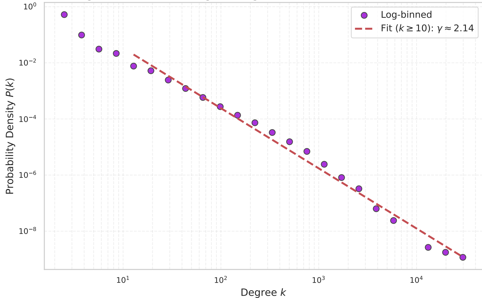
Degree Distribution (Log-Binning): Abe-Suzuki Network (5x5x5 km)
