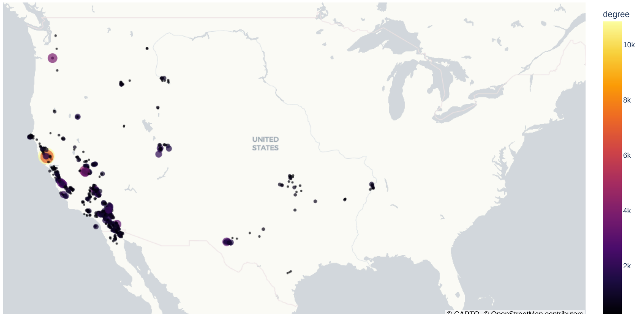
Abe-Suzuki Network Hubs: Top 2% Most Active Seismic Cells (10x10x10 km)
