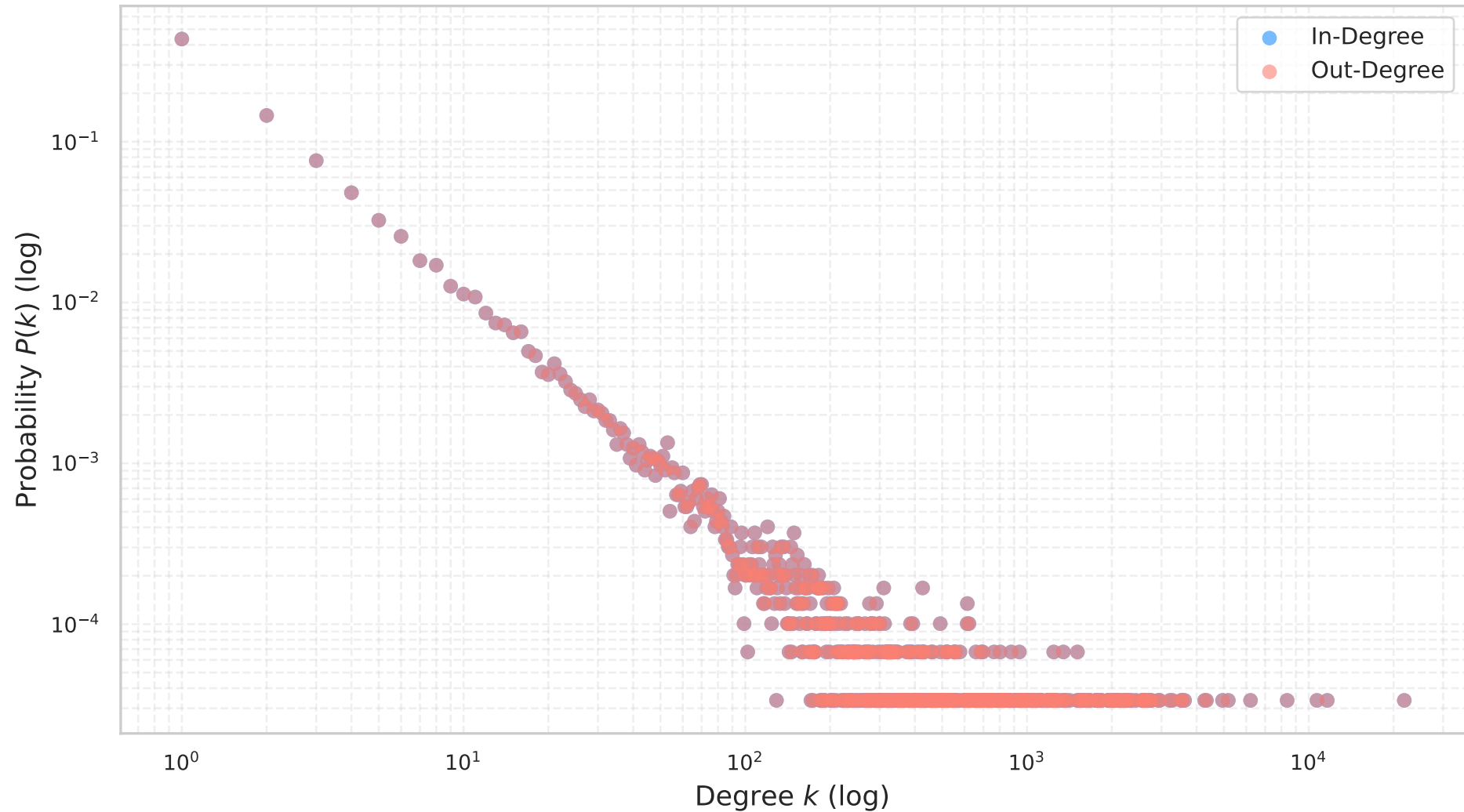
In vs Out Degree Distribution: Abe-Suzuki (10 km)
