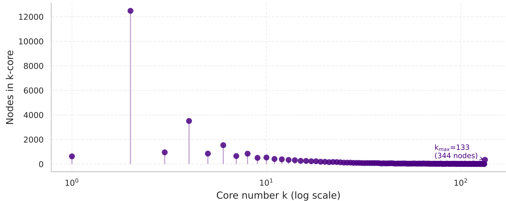
k-core Size Distribution — US (10 km)
