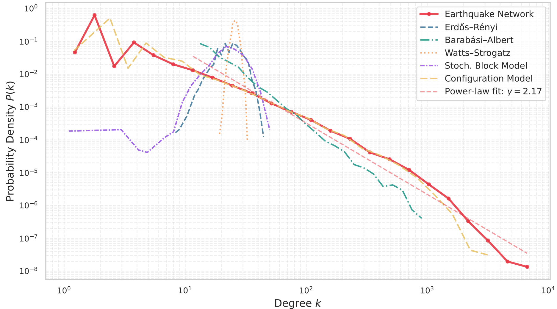
Degree Distribution vs Null Models: Abe-Suzuki US (10 km)
