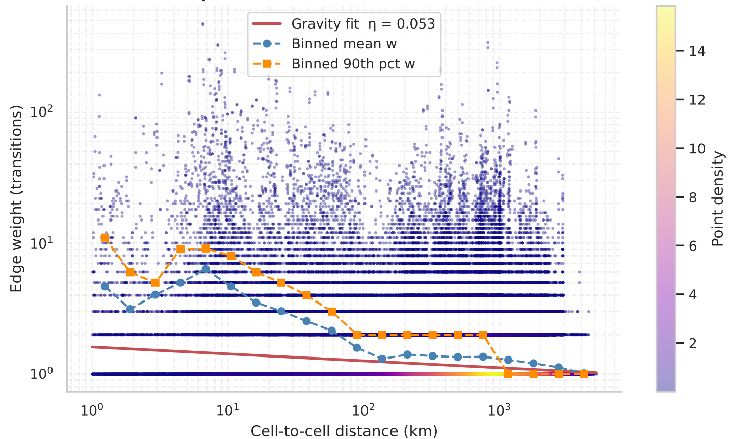
Distance Decay of Seismic Transitions — Abe-Suzuki US (10 km)
