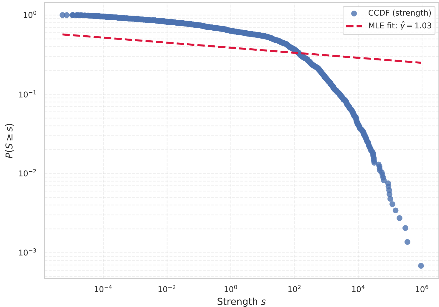
CCDF Strength Distribution: Abe-Suzuki Italy 10 km
