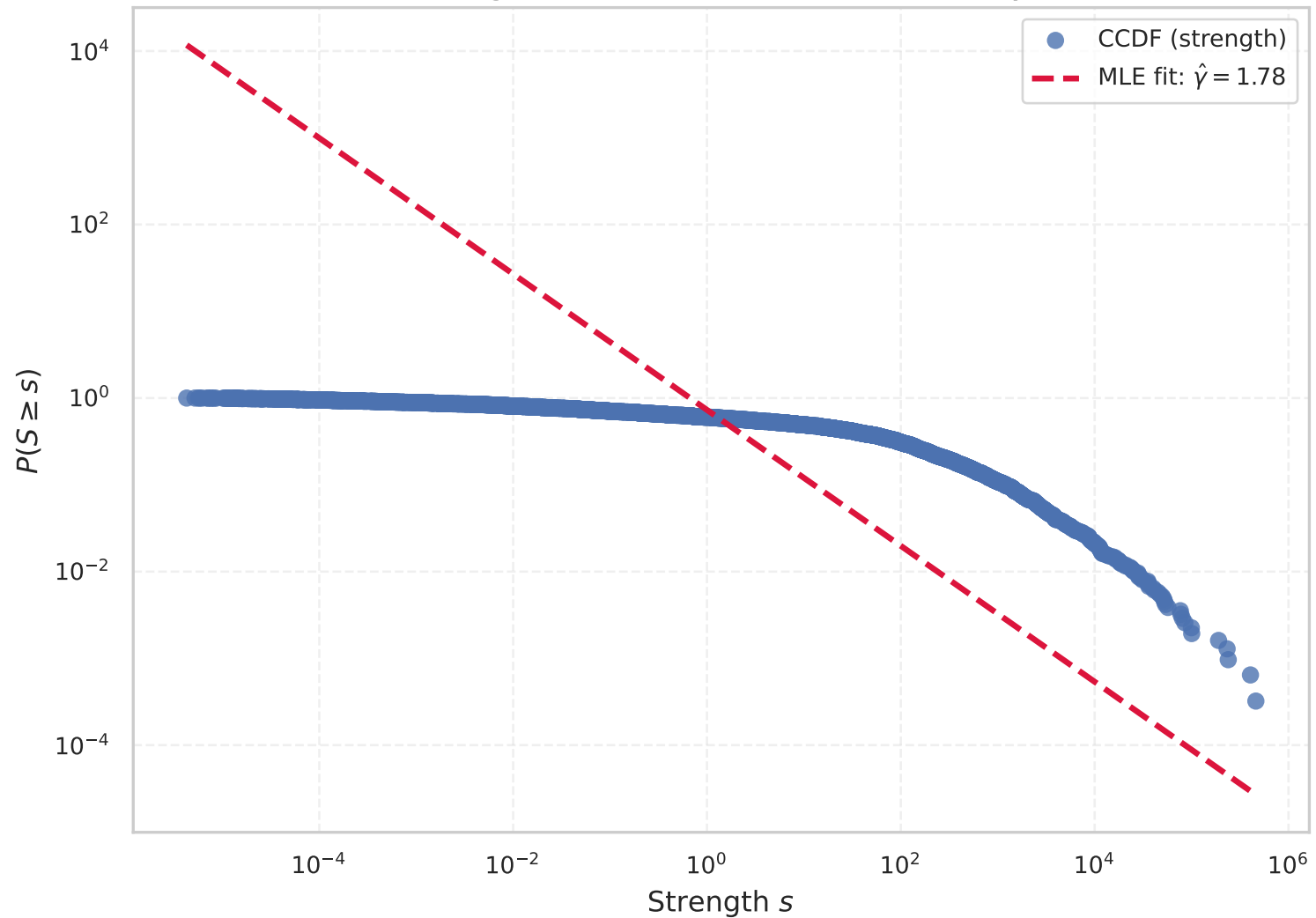
CCDF Strength Distribution: Abe-Suzuki Italy 20 km
