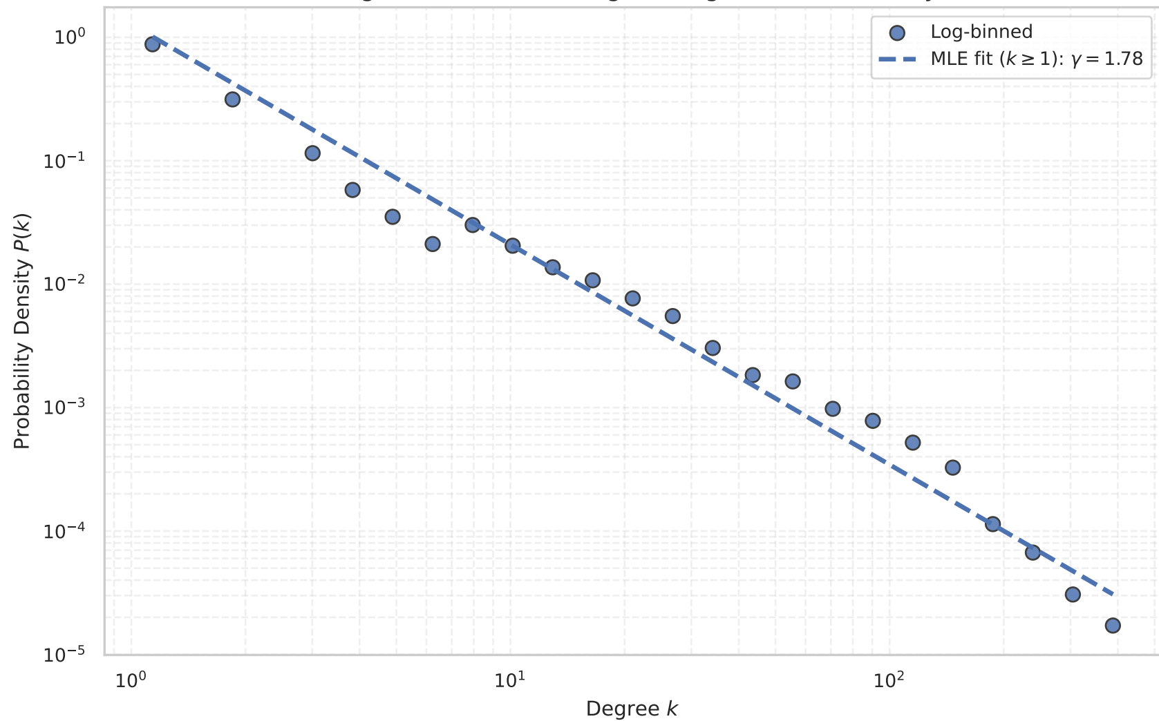
Degree Distribution (Log-Binning): Abe-Suzuki Italy
