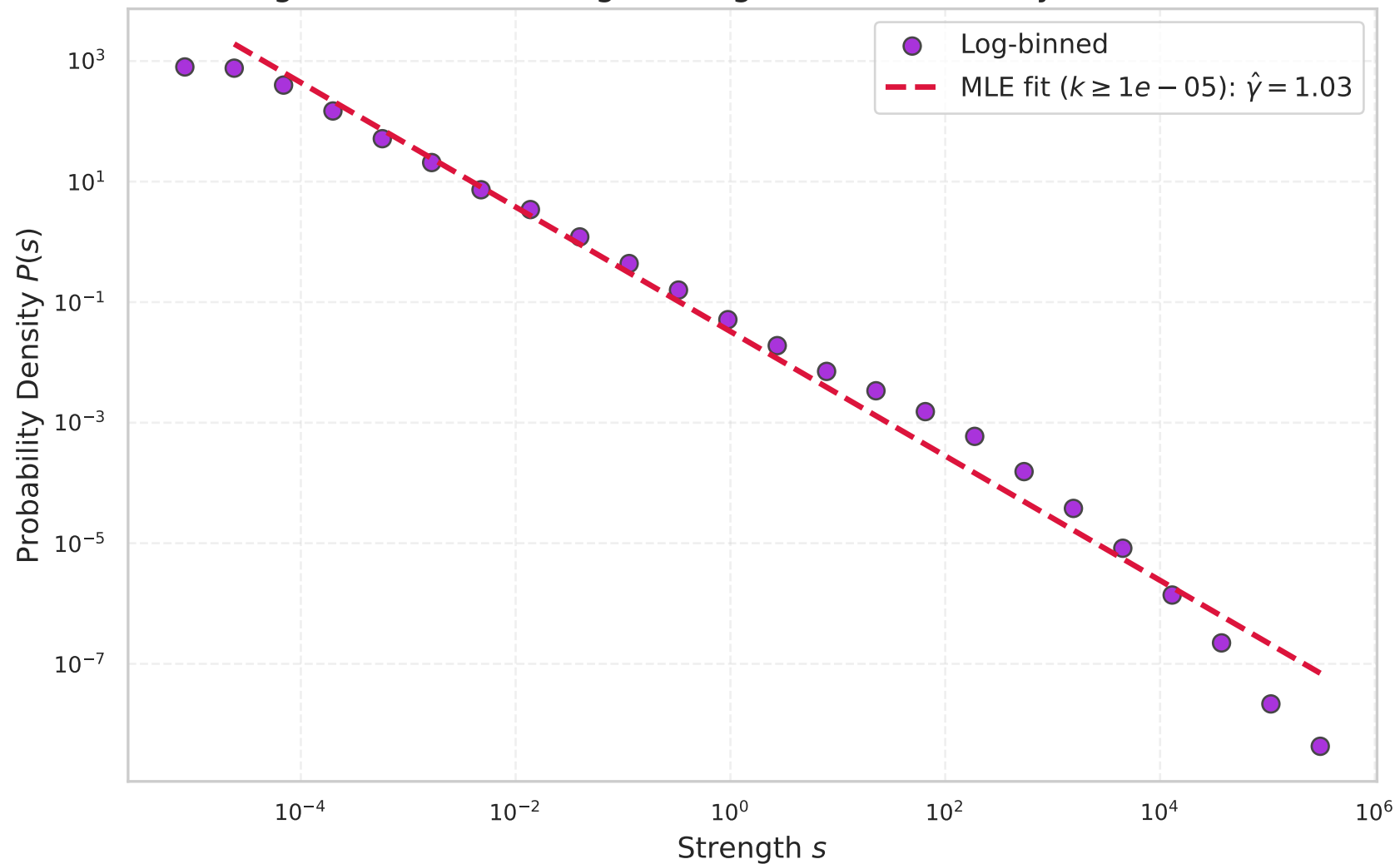
Strength Distribution (Log-Binning): Abe-Suzuki Italy (20x20x20 km)
