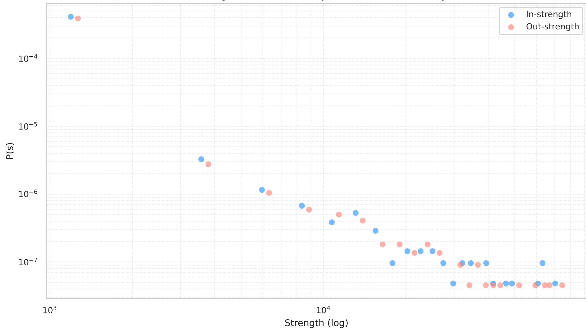
In vs Out Strength Distribution (Hybrid): Abe-Suzuki Italy (10 km)
