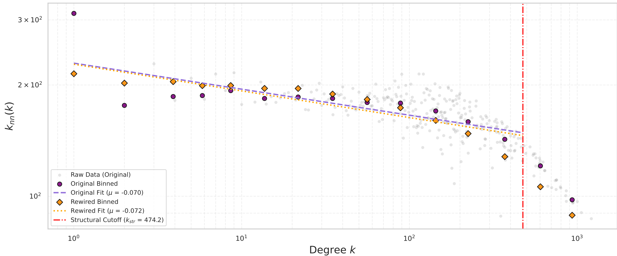
Assortativity Fit with Randomization Test
