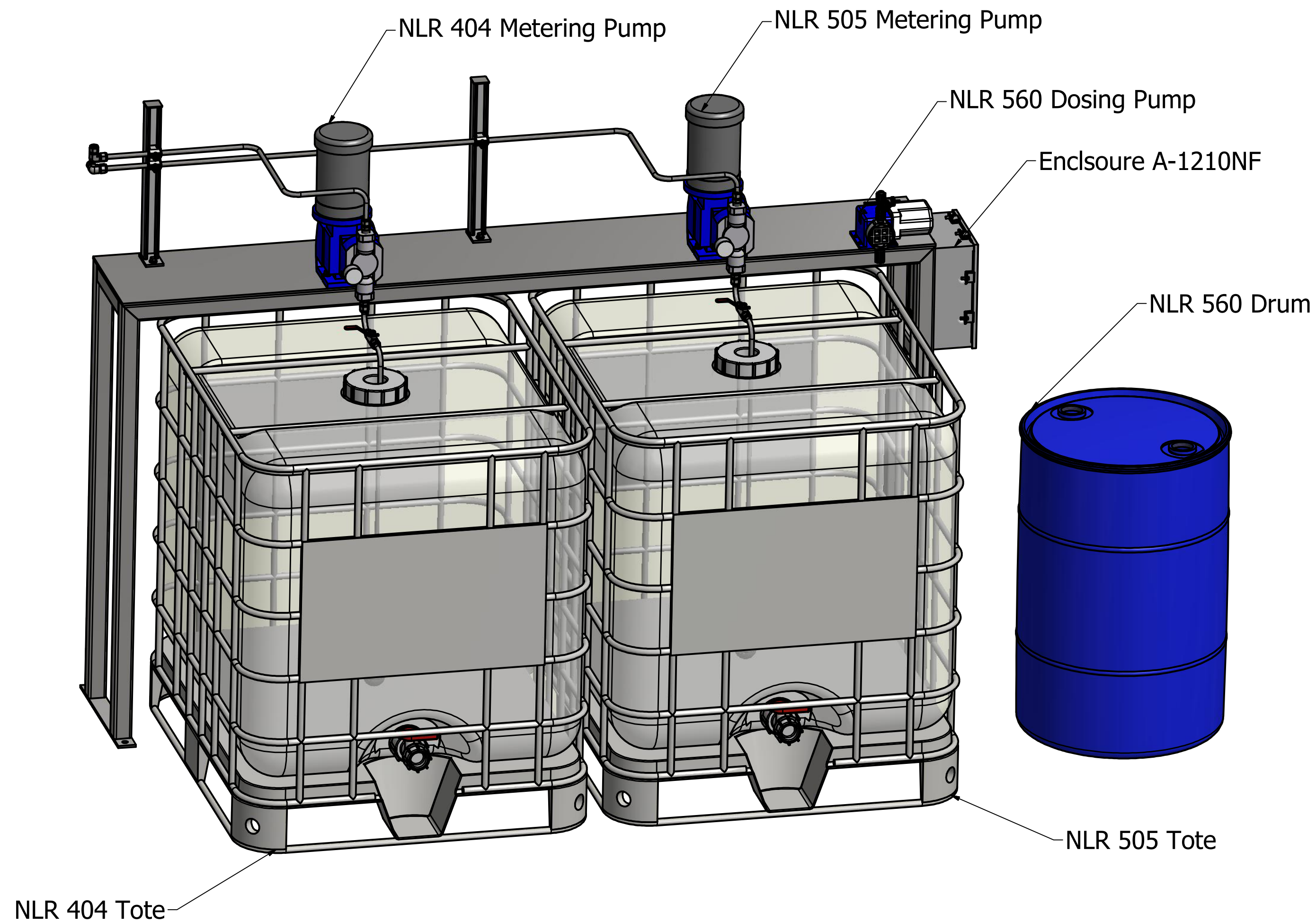
Standard Chemical Metering Station
