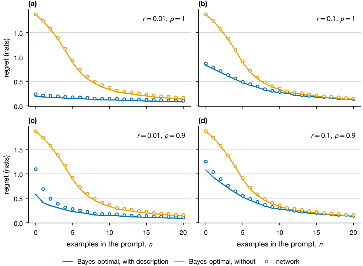
Figure 3: Networks trained on the matching distribution track the Bayes-optimal predictor, except on an unreliable description alone. Regret against the number of examples for the network (markers; standard errors over 20,000 prompts are smaller than the markers) and the Bayes-optimal predictor (lines), one training run per panel. In each panel the lower curve is prompts with a description followed by n examples and the upper curve is prompts with n examples alone; the ESS is the n at which the upper curve reaches the lower curve’s value at n = 0 . (a) r = 0.01, p = 1 ; (b) r = 0.1, p = 1 ; (c) r = 0.01, p = 0.9 ; (d) r = 0.1, p = 0.9 . In (c) and (d) the network’s regret with the description alone exceeds the Bayes-optimal predictor’s by 0.5 and 0.2 nats, and its ESS is 4.3 against 6.8 and 3.6 against 4.2.
