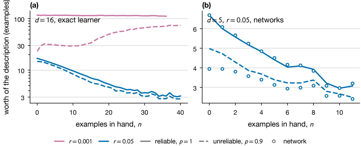
Figure 2: An unreliable description gains worth as examples verify it; a reliable one does not. Worth of the description with n examples in hand (Definition 2), as further examples saved. (a) Exact learner, d = 16 , a_0 = 10 , mean of three seeds of 2,000 prompts; log scale. (b) Trained networks at d = 5 , r = 0.05 (markers, one model per reliability) against the exact learner (lines). The network trained at p = 0.9 under-values its description alone and converges to the exact learner as examples arrive.
