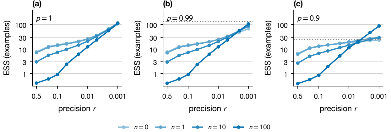
Figure 2: Reliability caps precision only while nothing can check the description. ESS of a description against its precision r with n examples in hand ( ESS_n of Definition 1), one panel per reliability; d = 16 , a_0 = 10 , log scales, one seed of 8,000 prompts. Dotted: the limit of the ESS alone as r \rightarrow 0 , 135 examples at p = 0.99 and 25 at p = 0.9 . Alone, the p = 0.9 description reaches 23 examples at r = 0.001 , close to that limit, while the reliable one keeps rising; with 100 examples in hand the three panels nearly coincide (109, 107, and 88 at r = 0.001 ).
