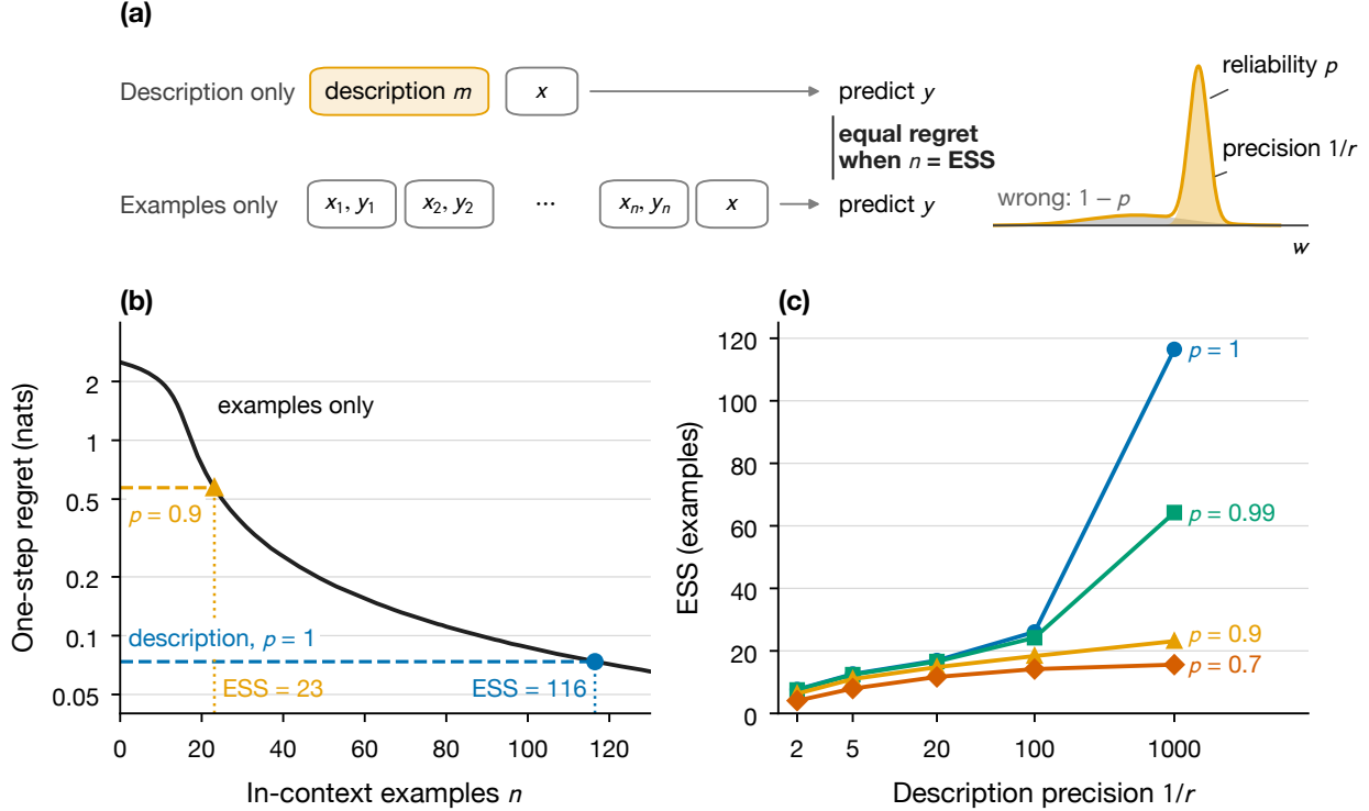
Figure 1: A task description is worth a number of in-context examples, set by its precision and capped by its reliability. (a) A Bayes-optimal predictor sees either a description or n examples; the description’s effective sample size (ESS) is the n at which their one-step log-loss regrets match. The description acts as a prior on the task w : with probability p (reliability) it is correct and leaves a fraction r of the prior variance (precision 1/r ); otherwise w follows the base prior (sketch, not to scale). (b) Regret after n examples (black) and regret of a description with r = 0.001 (dashed). The crossings give its ESS: 116 examples if it is always correct, 23 if it is correct 90% of the time. (c) ESS against precision. A reliable description keeps gaining from precision; an unreliable one saturates (Proposition 2). Panels (b, c): d = 16 , a_0 = 10 ; mean of three seeds, standard deviation at most 2% of each ESS.
