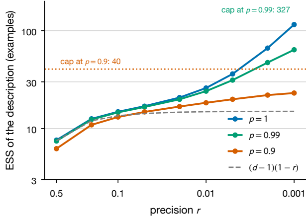
Figure 2: Precision pays linearly until the description is worth about d examples, and reliability caps it. ESS of a description alone against its precision at three reliabilities; d = 16 , a_0 = 10 , log scales, one seed. Dashed: (d - 1)(1 - r) of Proposition 1. Dotted: the cap of Proposition 2 at p = 0.9 .
