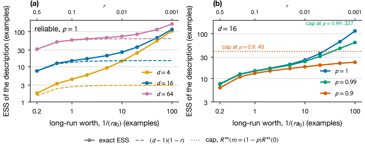
Figure 2: Precision pays linearly until the description is worth about d examples, and reliability caps it. ESS of a description alone against its precision, read as what it is worth in the long run, 1/(ra_0) ; a_0 = 10 , log scales, one seed. (a) Reliable descriptions at d = 4, 16, 64 against (d-1)(1-r) of Proposition 1 (dashed). (b) d = 16 at three reliabilities; the dotted line is the cap of Proposition 2 at p = 0.9 .
