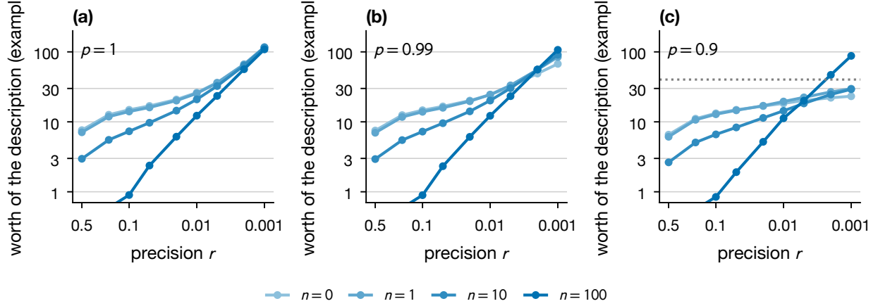
Figure 2: Reliability caps precision only while nothing can check the description. Worth of a description against its precision with n examples in hand ( \text{ESS}_n of Definition 1), one panel per reliability; d = 16 , a_0 = 10 , log scales, one seed of 8,000 prompts. Dotted: the cap of Proposition 2 at p = 0.9 with no examples. Alone, the p = 0.9 description saturates at 23 examples while the reliable one keeps rising; with 100 examples in hand the three panels nearly coincide (109, 107, 88 at r = 0.001 ).
