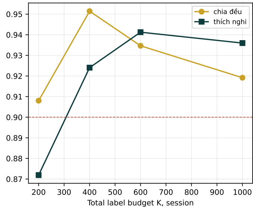
Average Coverage
