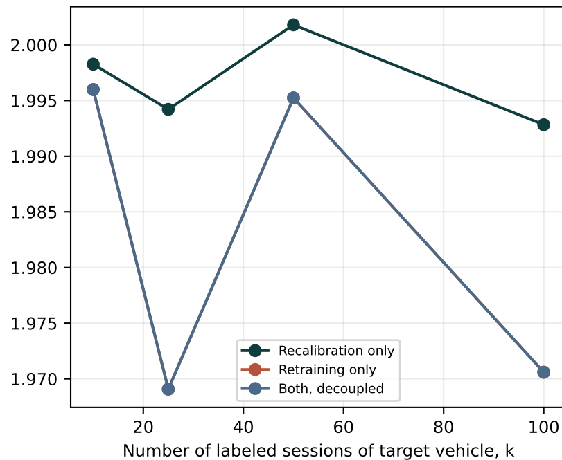
RMSE on target vehicle, Ah
