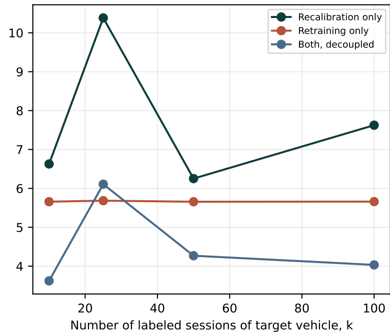
Interval width, Ah
