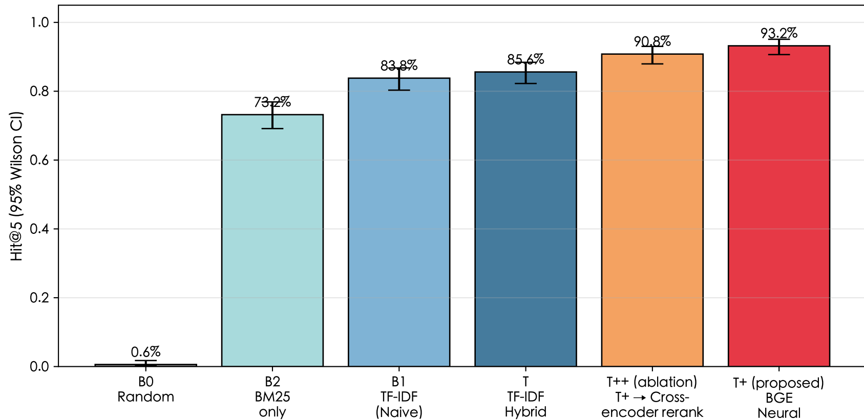
Fig. 2. Hit@5 across 6 Conditions (Test Set, n=500)
