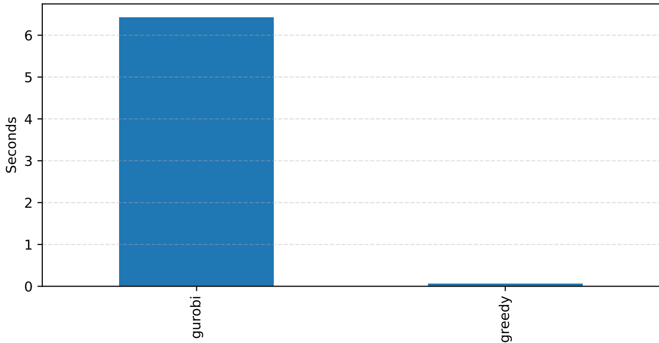
Running time: Gurobi vs Greedy
