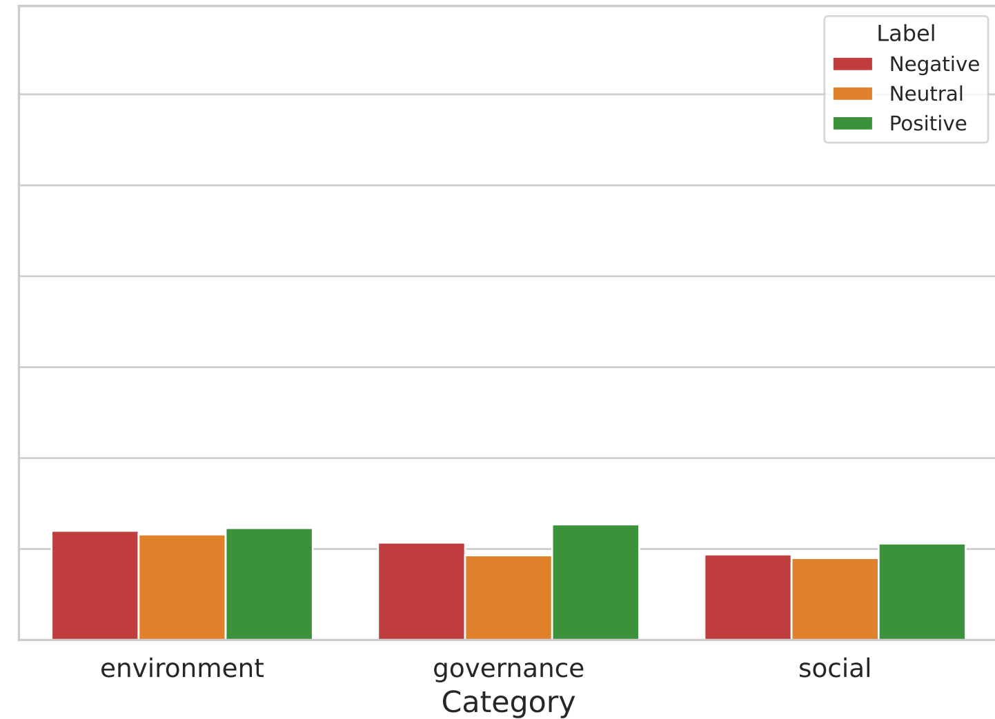
Test Dataset
