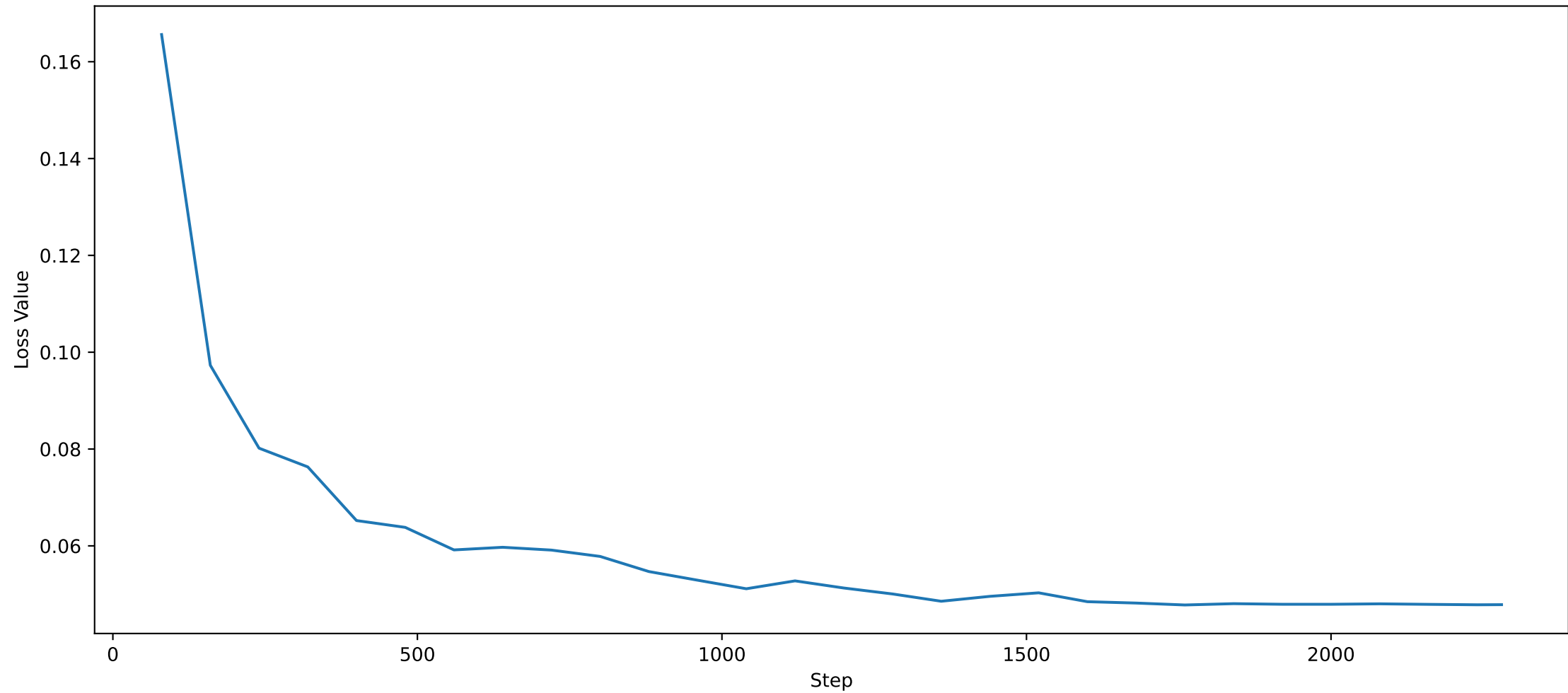
Evaluation Loss vs Step
