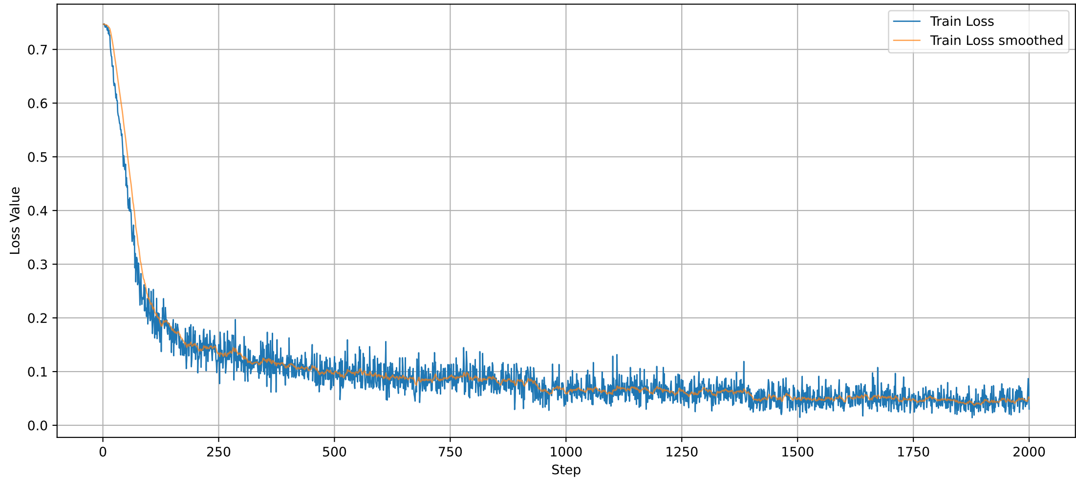
Training Loss vs Step
