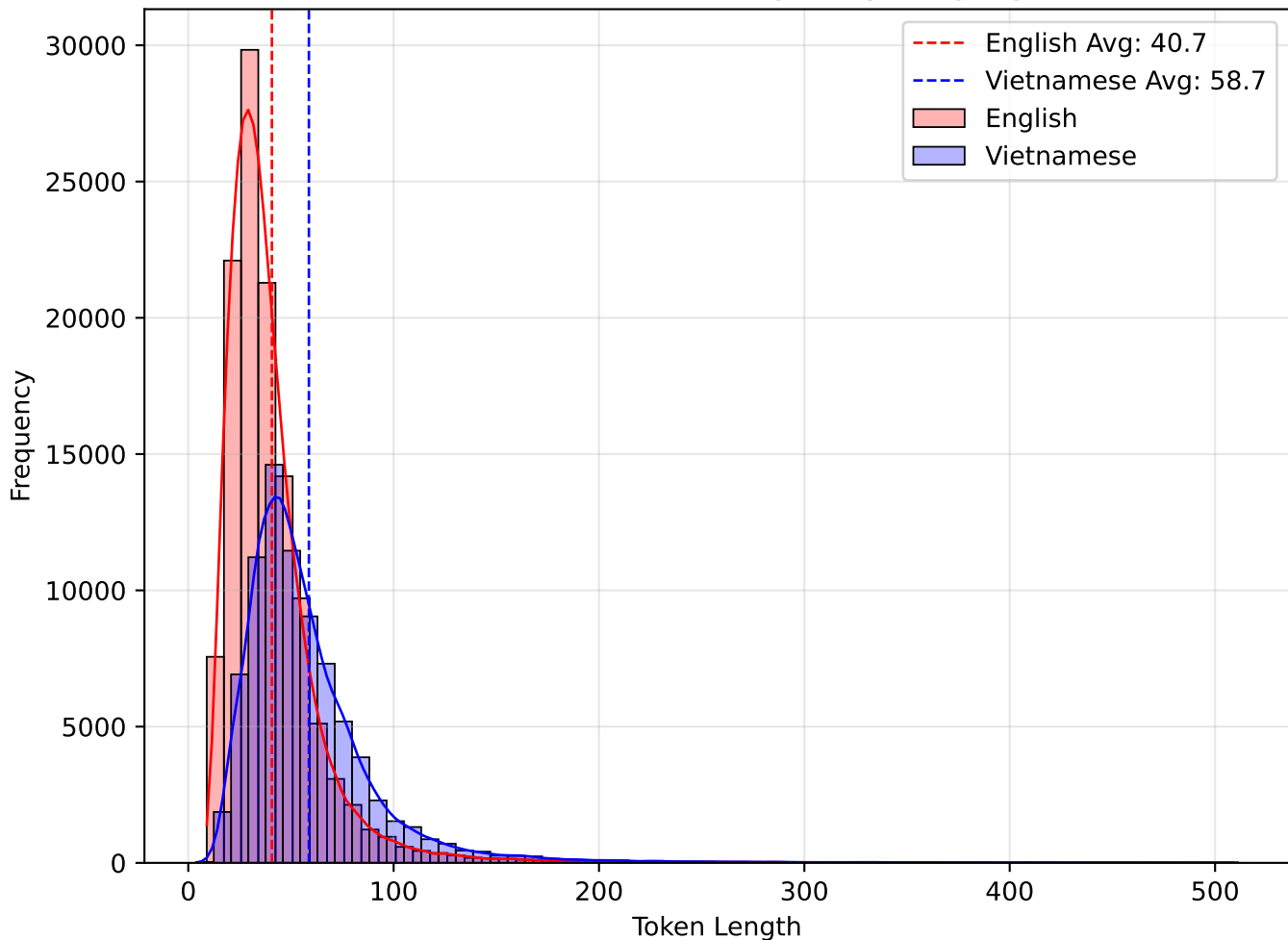
Distribution of Token Lengths by Language
