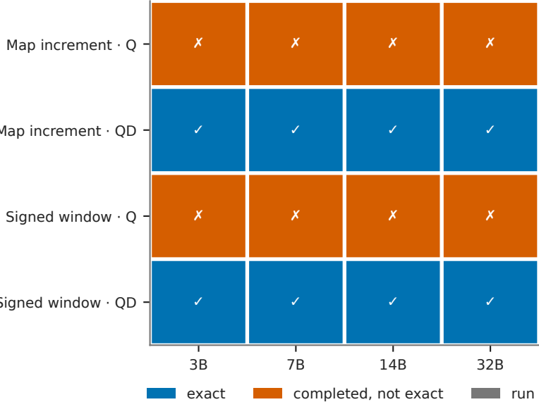
Training exact discovery
