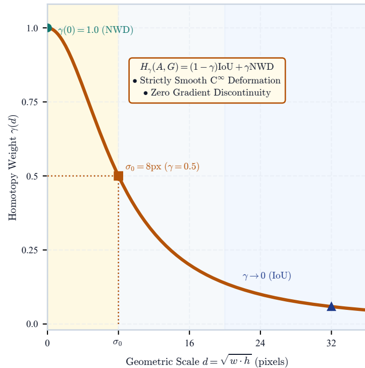
(c) Continuous Homotopy Deformation
