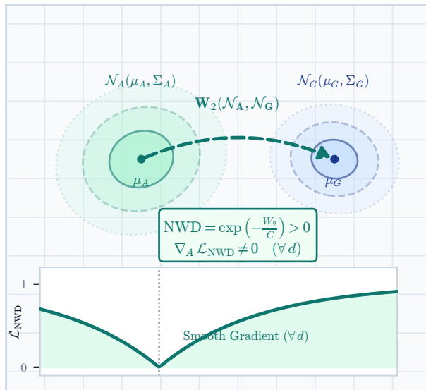
(b) Gaussian Optimal Transport
