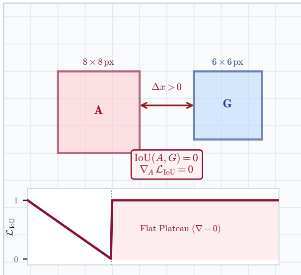
(a) Standard IoU Metric Collapse
