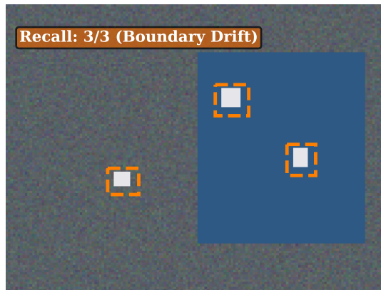
NWD (NeurIPS'21)
