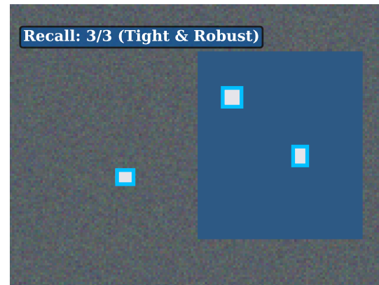
H-WIoU (Proposed)
