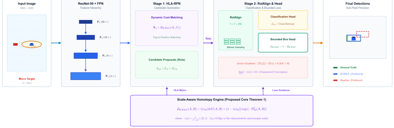
Figure 3: End-to-End Pipeline and Architecture of the Proposed Homotopy Wasserstein-IoU (H-WIoU) Detector. Multi-scale feature pyramids ( P_2 – P_5 ) extract spatial representations. In Stage 1, the Region Proposal Network (RPN) employs Homotopy Label Assignment (HLA) to compute continuous scale-adaptive similarity scores S_{H-WIoU} . In Stage 2, candidate RoIs are pooled via RoIAlign and supervised using the bounded Homotopy Regression Loss L_{H-WIoU} . The continuous scale homotopy parameter \gamma(s) = \frac{s^2}{s^2 + \sigma_0^2} smoothly deforms between pure optimal transport ( \mathcal{W}_2 ) under microscopic scales and discrete Lebesgue measure (IoU) for larger targets.
