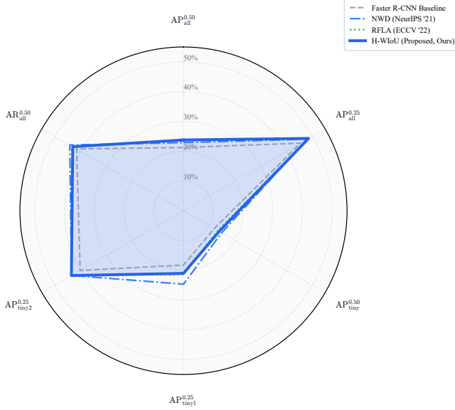
Figure 2: Multi-Metric Radar Comparison on TinyPerson Official Test Set. H-WIoU (blue) achieves the best overall AP_{all}^{0.50} (23.77%) and AP_{all}^{0.25} (48.58%) precision across competing paradigms, while remaining highly competitive on microscopic scale partitions and recall-focused axes.
