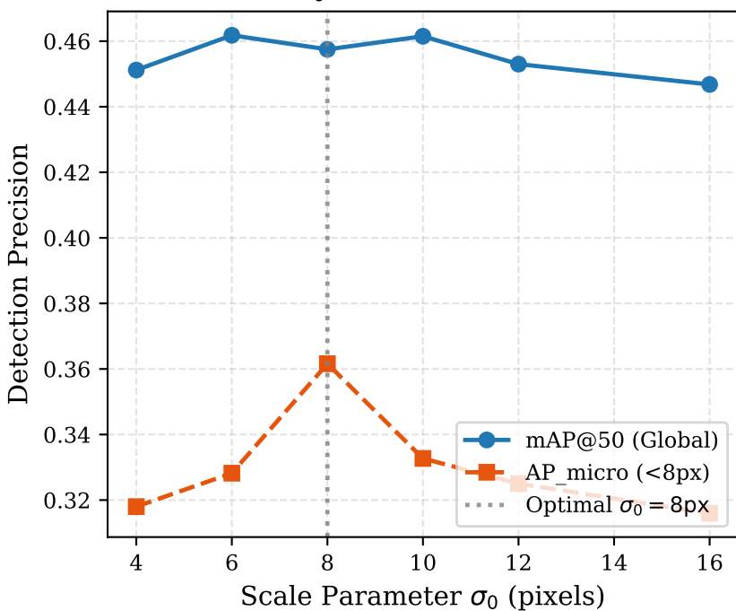
(a) Sensitivity to Characteristic Scale \sigma_0
