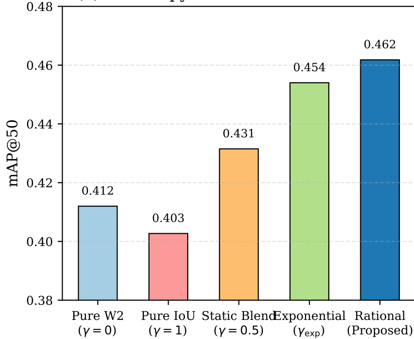
(b) Homotopy Deformation Formulation
