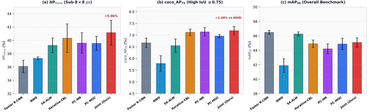
Figure 3: Statistical Performance Comparison across 21 Trained Models. Error bars denote \pm 1 std over 3 matched random seeds. (a) On microscopic instances ( AP_{\text{micro}} ), our Joint Model achieves a dramatic +5.06% gain over Vanilla Faster R-CNN. (b) In high-IoU localization ( coco\_AP_{75} ), our method outperforms NWD by +1.40% absolute (+24.2% relative improvement). (c) Overall mAP_{50} benchmark performance remains high and competitive.
