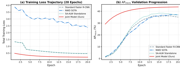
Figure 4: Training Dynamics and Convergence Trajectories. (a) Total training loss progression over 20 epochs. (b) Validation AP_{\text{micro}} trajectory, showing rapid and stable tiny-object convergence in our proposed Joint framework compared to standard baselines.
