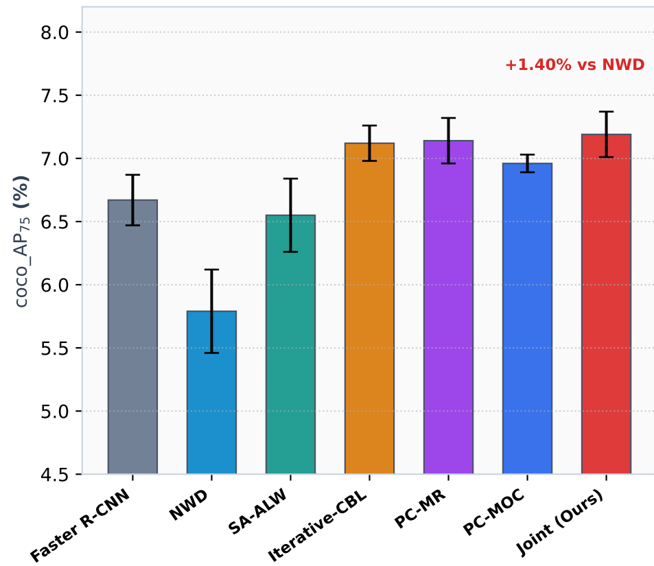
(b) coco_AP 75 (High IoU ≥ 0.75)
