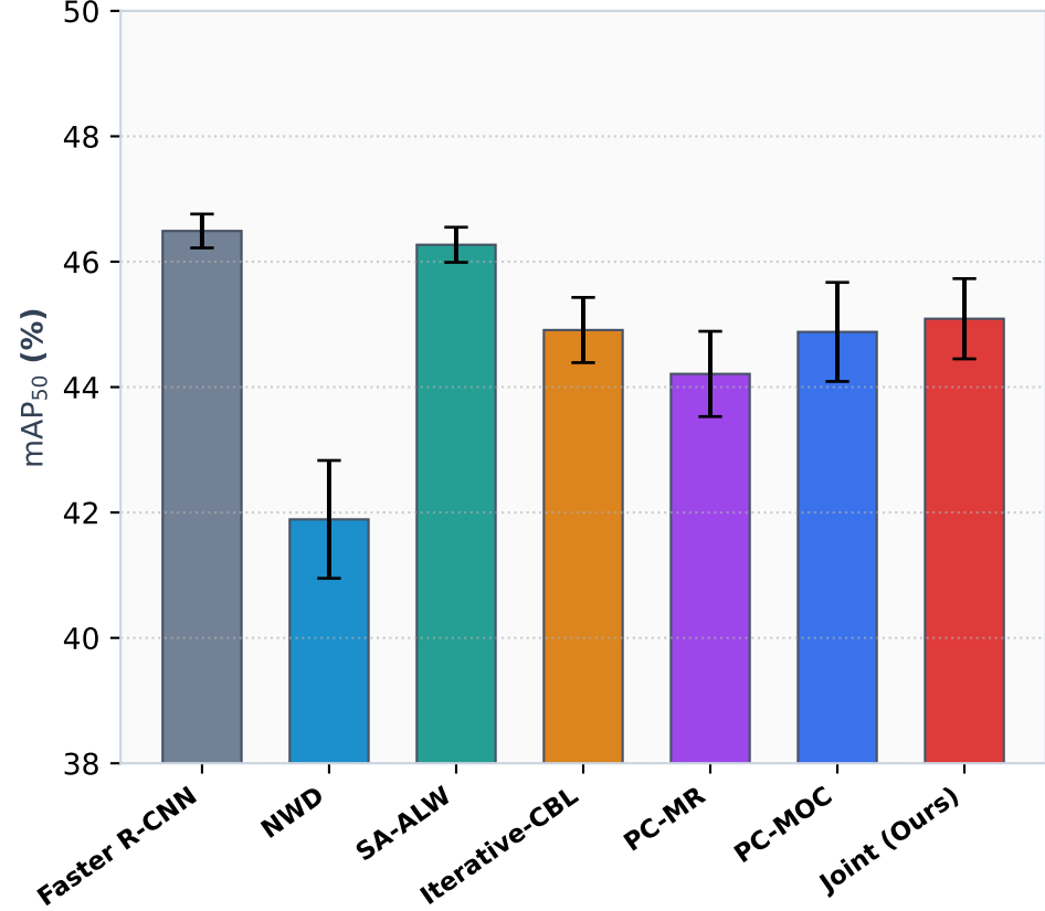
(c) mAP 50 (Overall Benchmark)
