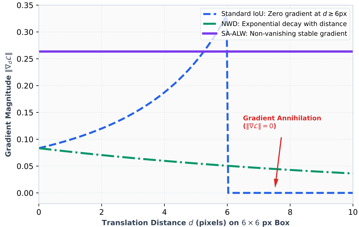
(b) Gradient Magnitude \|\nabla_d \mathcal{L}\| vs. Offset
