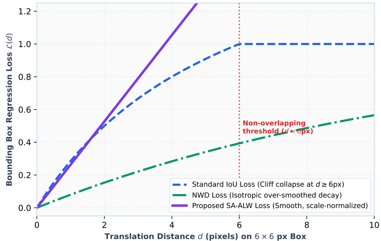
(a) Loss Function Value vs. Positional Offset
