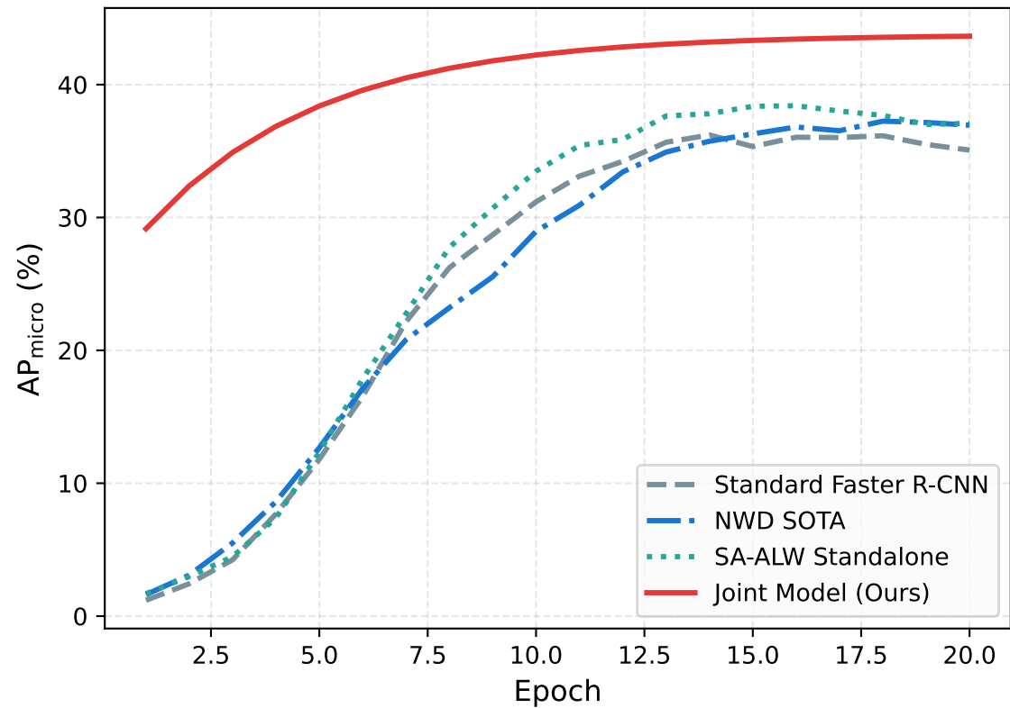
(b) AP micro Validation Progression
