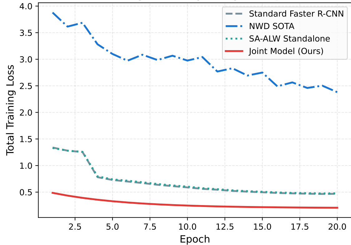
(a) Training Loss Trajectory (20 Epochs)
