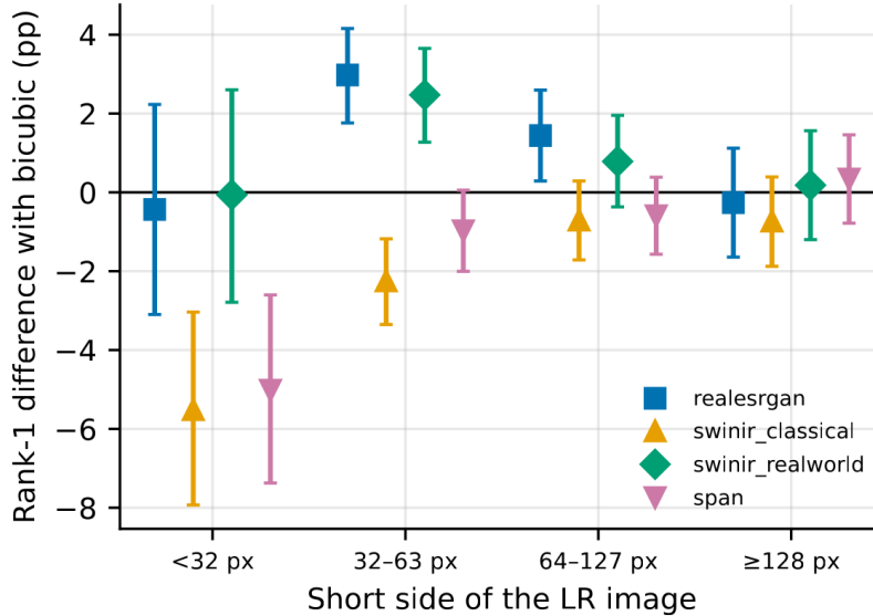
Figure 2: D1: Rank-1 difference with bicubic by short side of the LR image, with 95% bootstrap intervals over test images; hollow markers are bins with fewer than 50 test images (not tested); none occur in D1.
