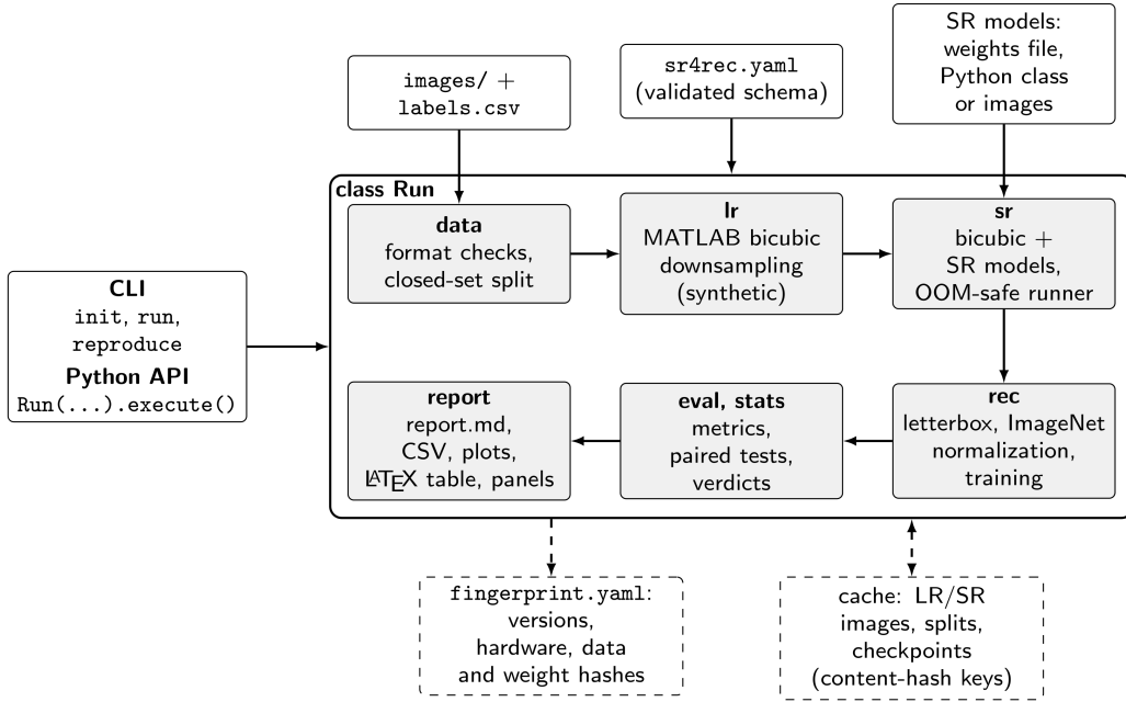
Figure 1: Architecture of SR4Rec. The CLI and the Python API share one Run class; expensive steps are cached under content-hash keys; every run writes a report and a fingerprint.
