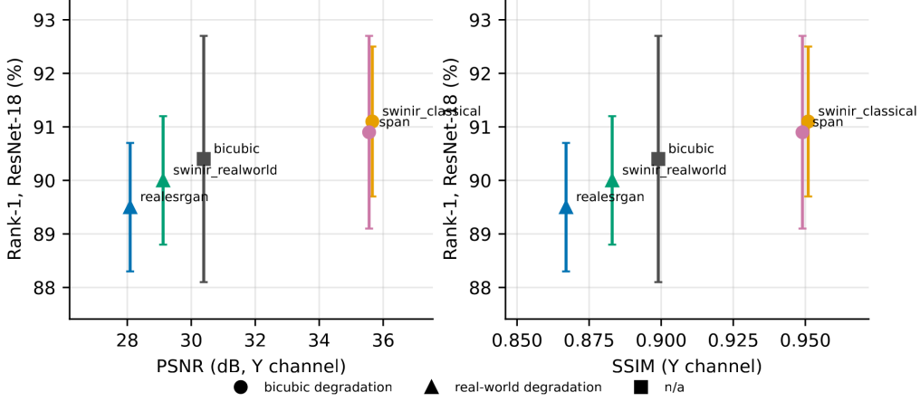
Figure 3: D2: PSNR and SSIM of each SR model against Rank-1 (mean \pm sd over seeds); marker shape gives the degradation the model was trained for.
