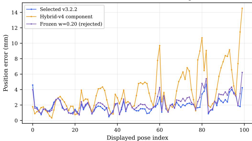
(c) Position error — no smoothing
