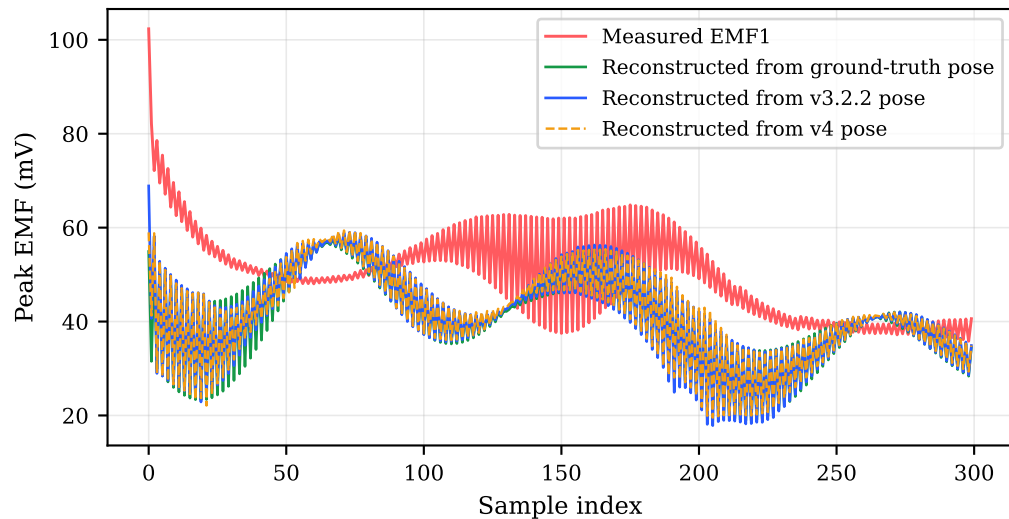
(a) EMF1 reconstruction
