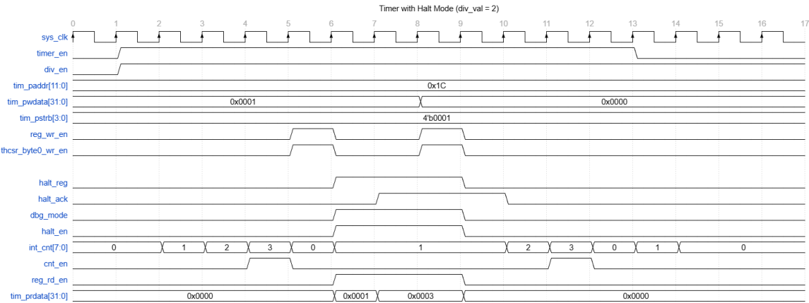
Figure 4: Counter Control timing
