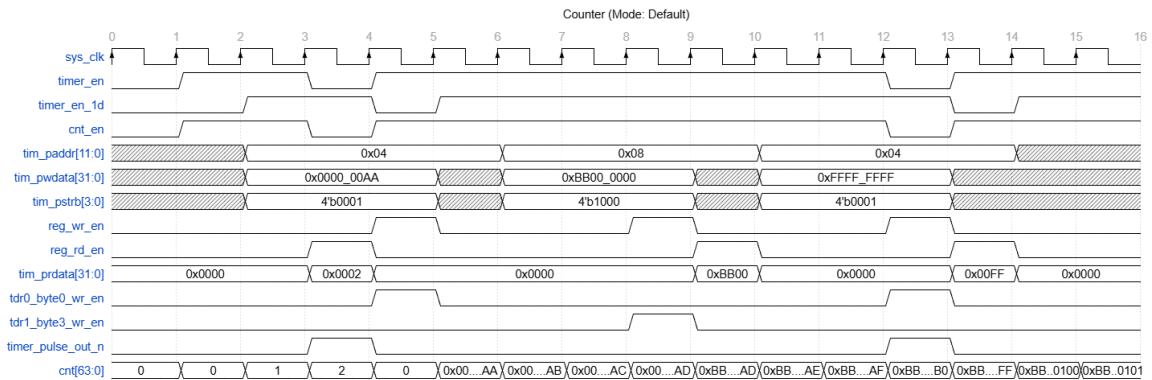
Figure 8: Counter timing
