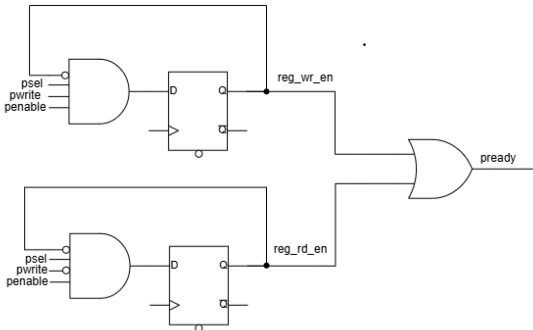
Figure 3: APB Slave logic diagram
