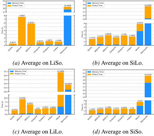
Figure 4. Time consumption of different LLMsys in off-policy experiments on four task-format-base partitions of MemoryBench. The bars show the average time per case for memory operations (Memory Time, in blue) and prediction on the test set (Predict Time, in orange), measured in seconds. Note that the construction of memory indexes or retrieval indexes are also considered as a part of the Memory Time. More details can be found in A.3.8.
